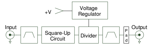
LNPDN Block Diagram
