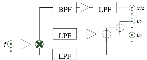
LNRD Block Diagram
